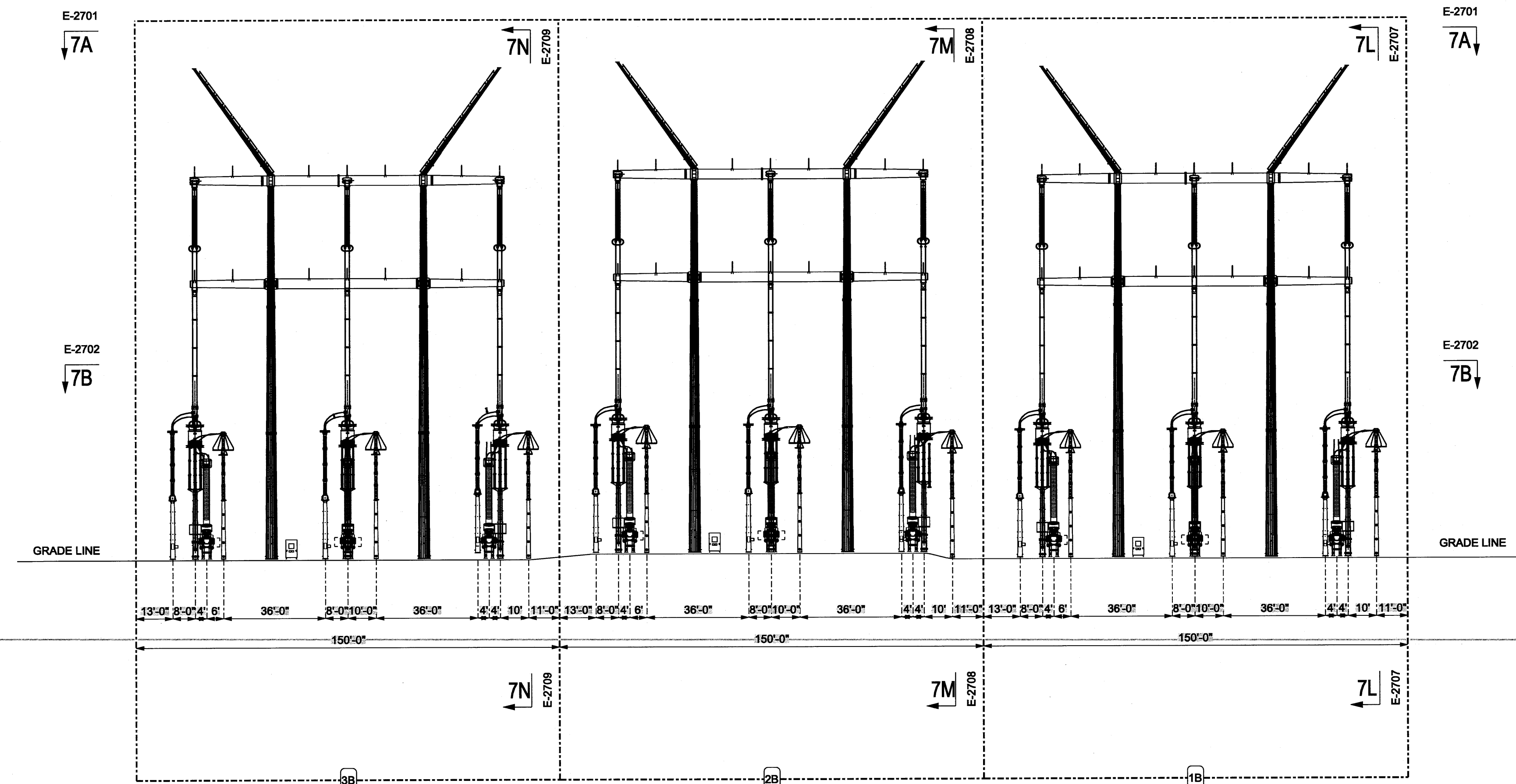
SECTION '7F-7F'
