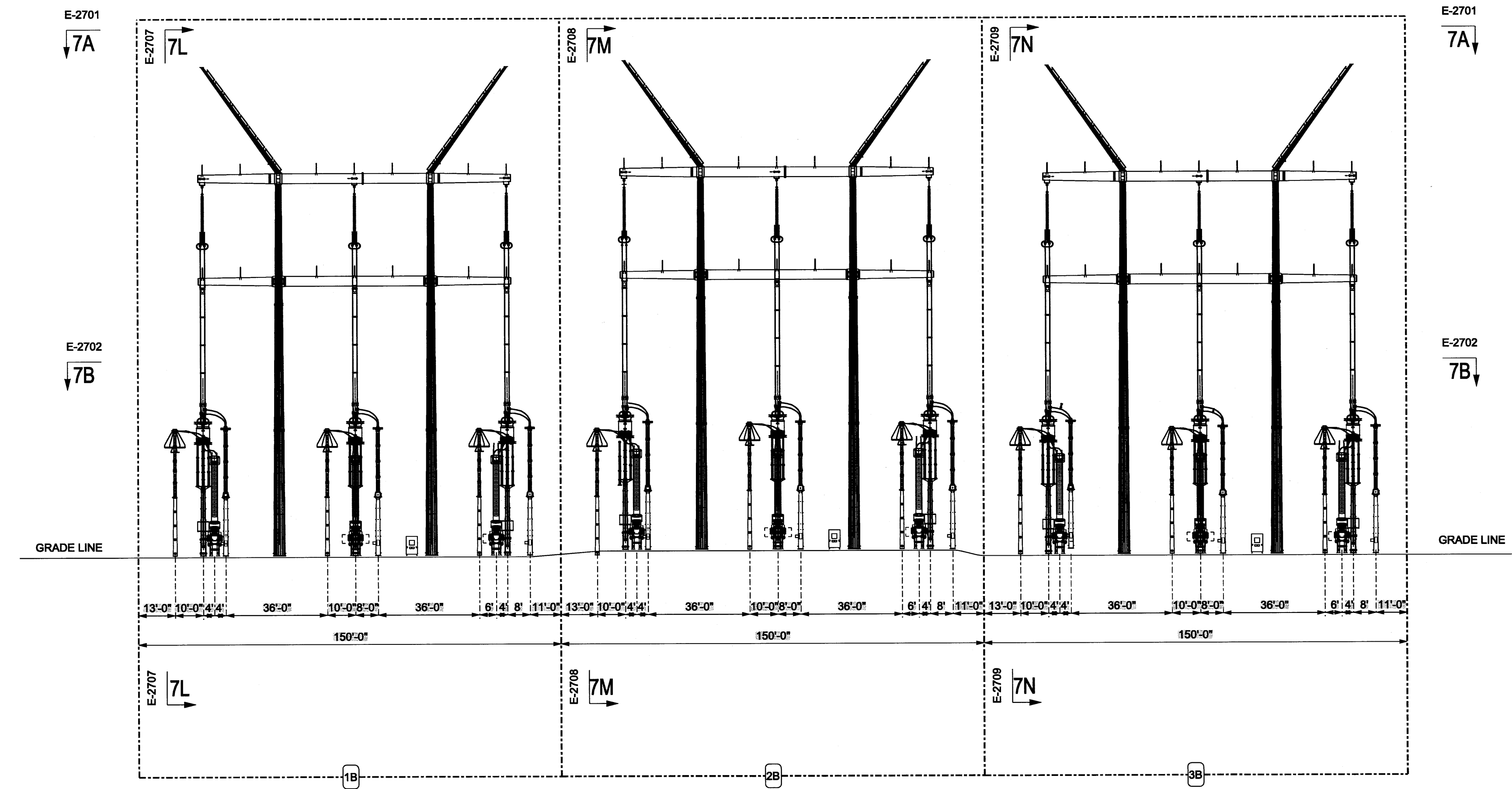
SECTION '7G-7G'
