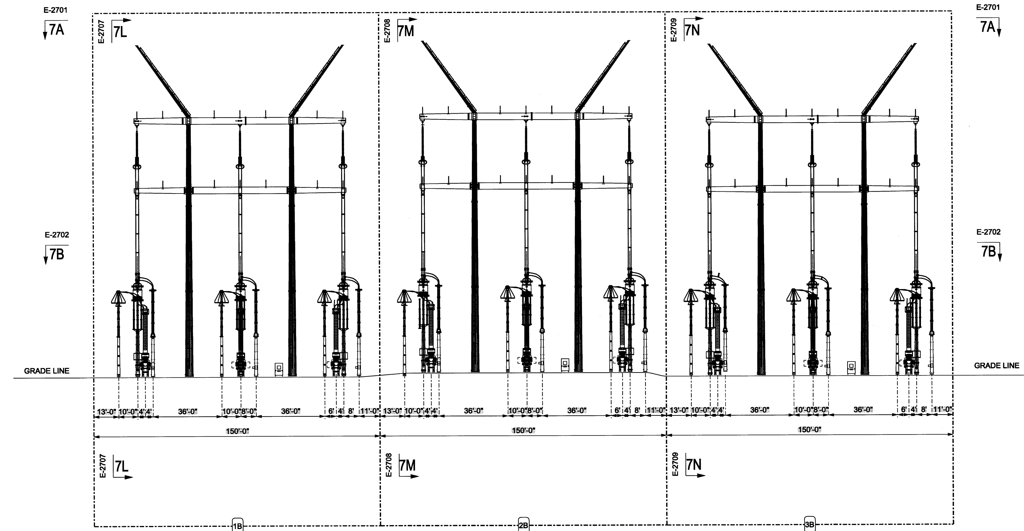
SECTION '7G-7G'
