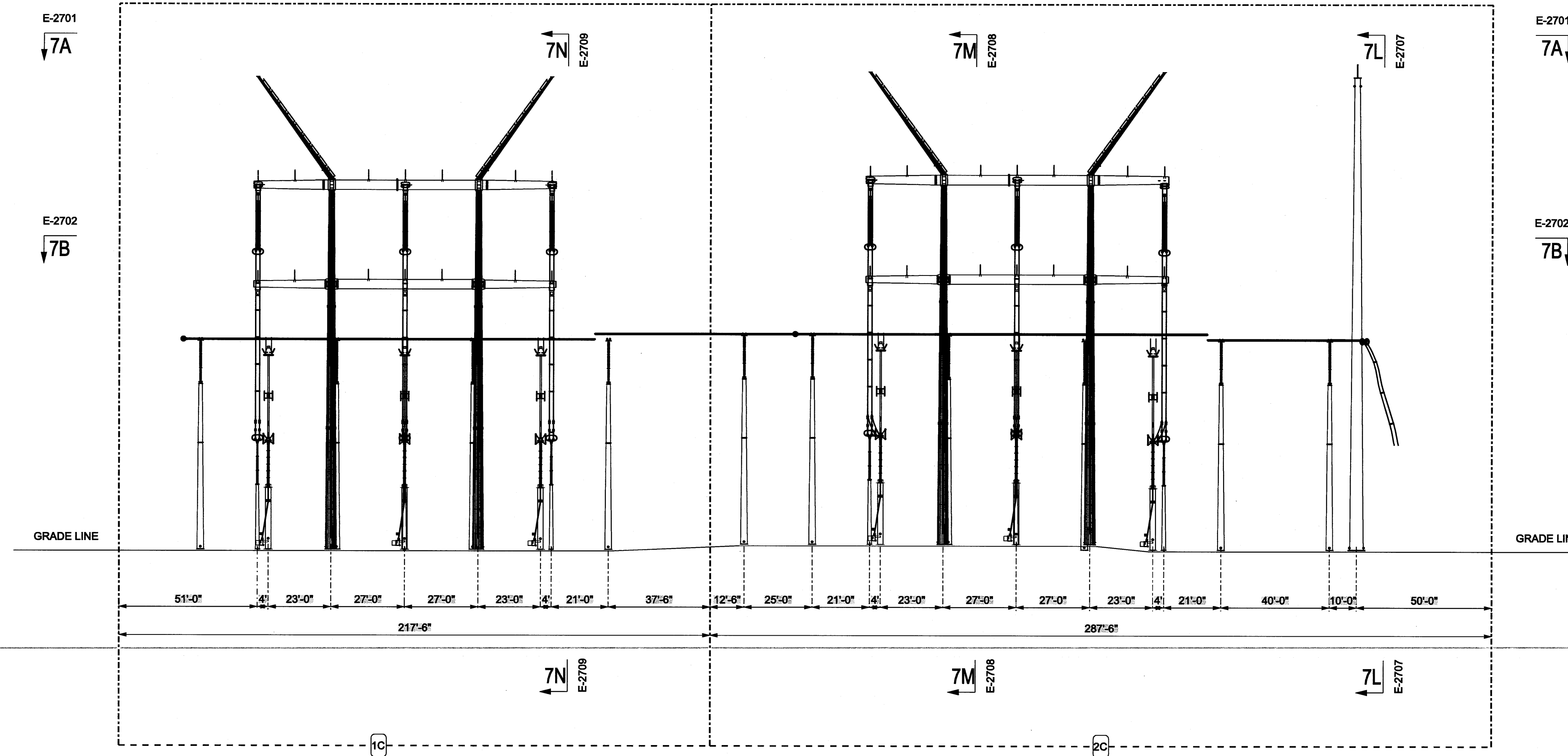
SECTION 7J-7J
