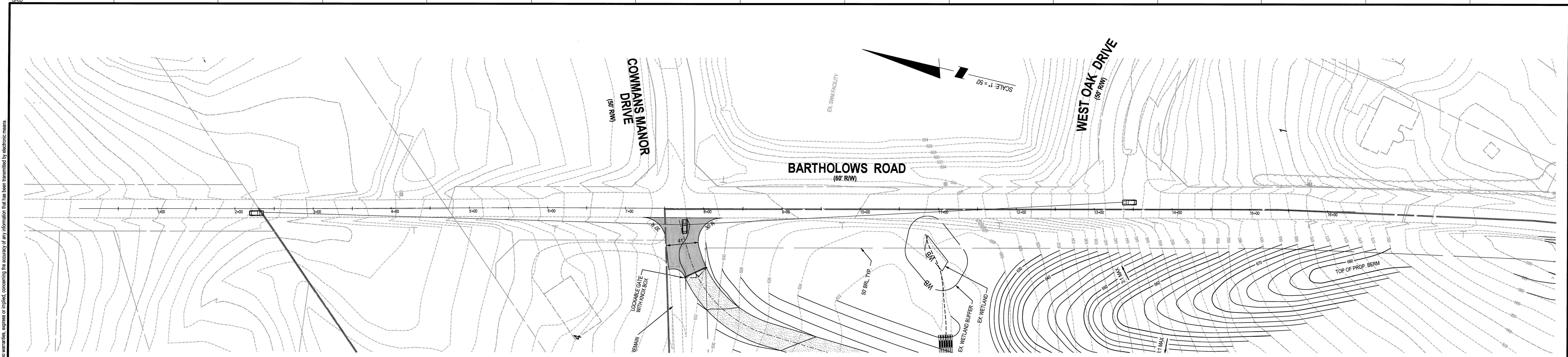
BARTHOLOWS ROAD PLAN VIEW
